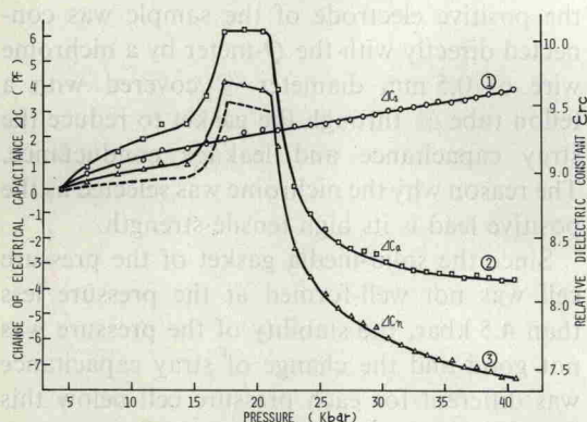
Fig. 2. The measurements of capacitance for a sample of \text{CaCO}_3 and the pressure dependence of relative dielectric constant along c -axis ( \epsilon_{rc} ) at 24°C. Curve ①, ② and ③ show change \Delta C of stray capacitance of the lead, capacitance of the sample with lead and the sample itself, respectively. The dotted line indicates a corrected curve of ③ in the phase I and II of \text{CaCO}_3 . (The scale on the left side is available for all curves and the scale on the right side for the curve ③ only.)
